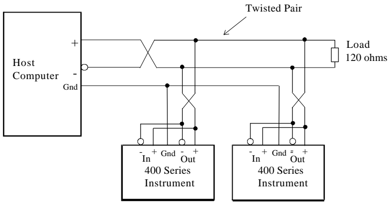
Figure 2 RS485 Interface
