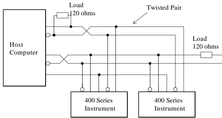
Figure 1 RS422 Interface
